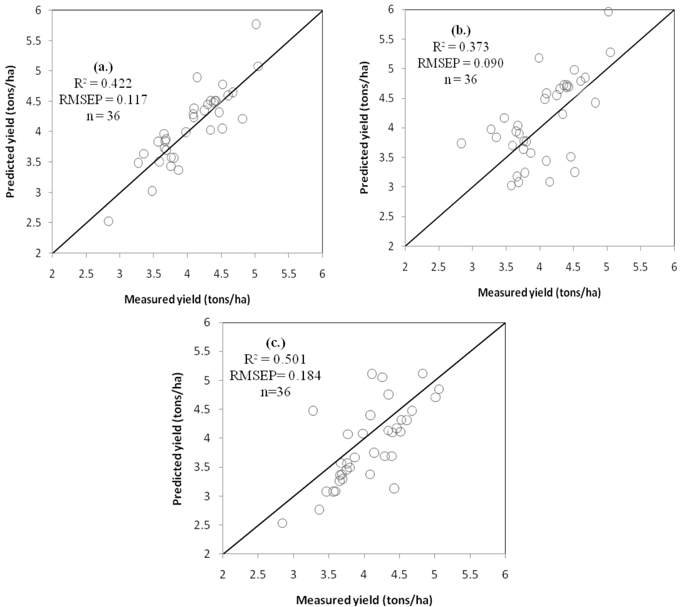
Figure 7: One-to-one relationship between predicted and measured maize yields from June images over Cairo using individual selected indices for Cairo (a) = NDVI, (b) = SAVI and (c) = VI
