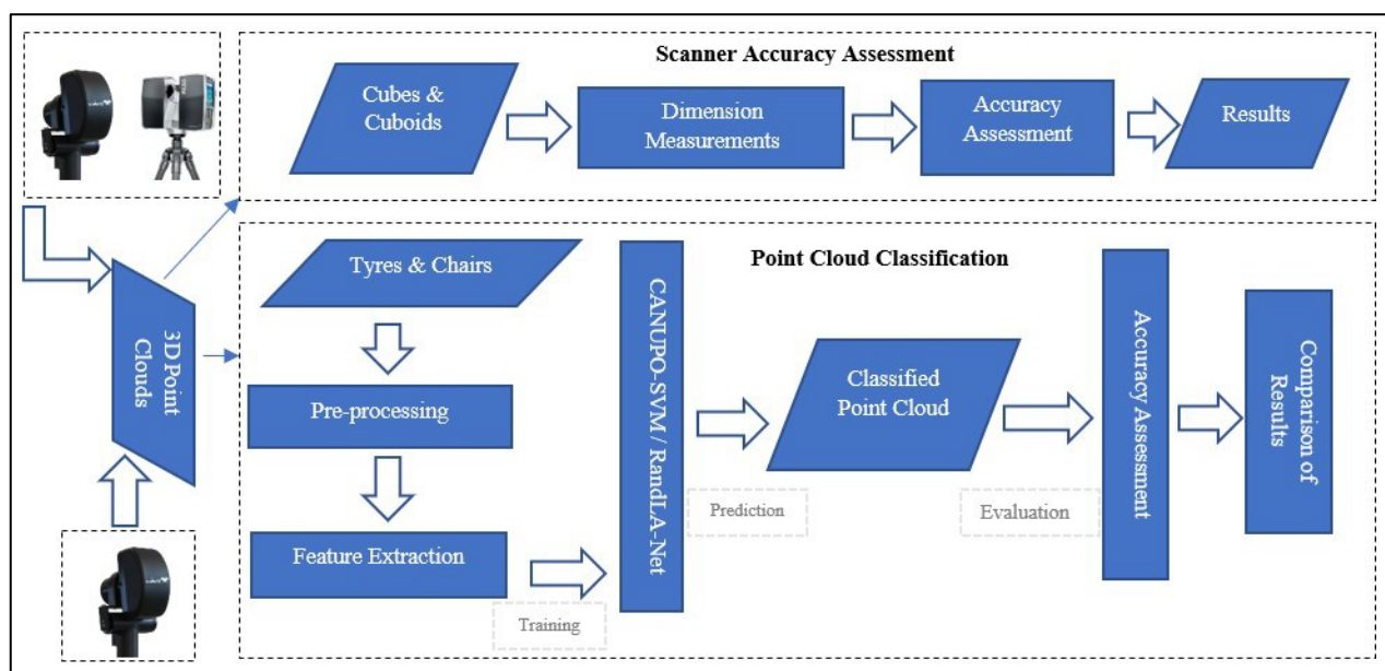
Figure 3: Flow chart showing the overall methodology workflow: accuracy assessment and point cloud classification.
