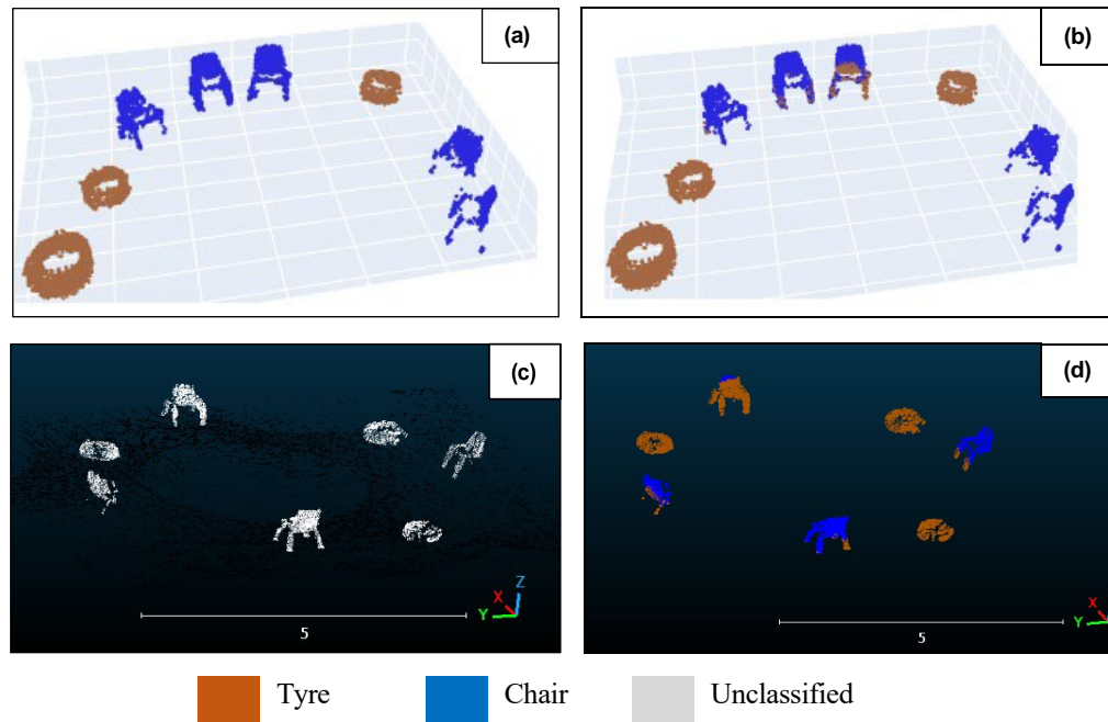
Figure 7: Classification results of the RandLA-Net Model: (a) Validation dataset, (b) Classified validation dataset, (c) Test dataset and (d) Classified test dataset.
